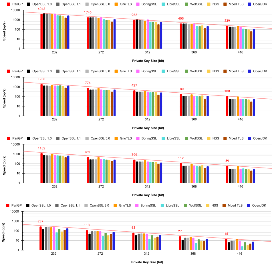
FIGURE 10. DHE public key generation speed - small exponent 232-416 bits.
