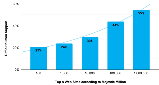
FIGURE 1. Diffie–Hellman support in the Top 1 million domains.
